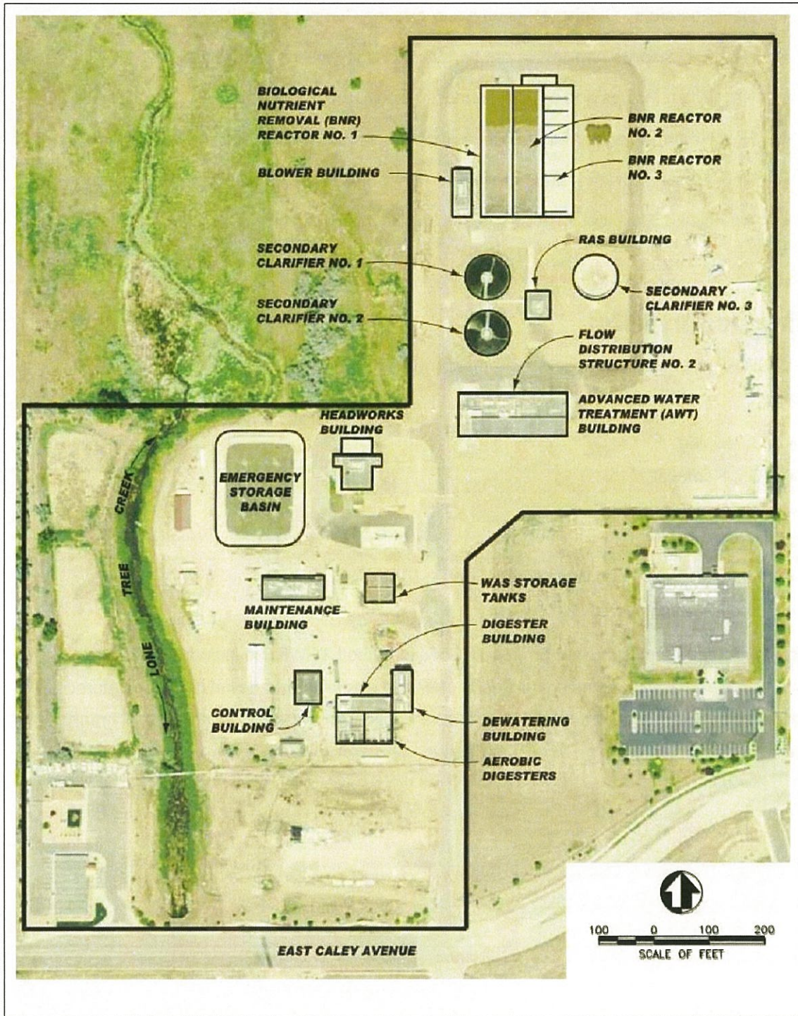
FIGURE 1 ACWWA LONE TREE CREEK WATER REUSE FACILITY SITE LAYOUT
